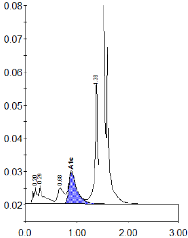
Peak table - ID: 10420415
